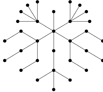
#8: 0123^3(1(23)^3)^2(12^4)^2 1 .
