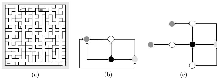
Fig. 2: A maze (a) and its path- and CoPa-minimal models ((b) and (c))
