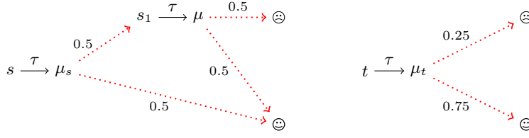
■ Figure 3 Probabilistic weak bisimulation is too strong.
