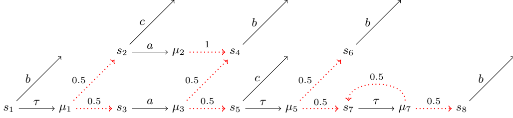
■ Figure 1 Example probabilistic automaton \mathcal{A} .
