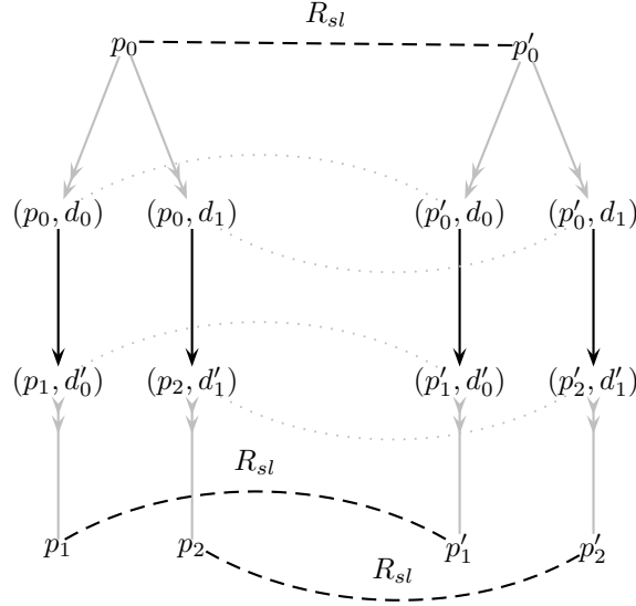
Figure 3: Stateless Bisimilarity
