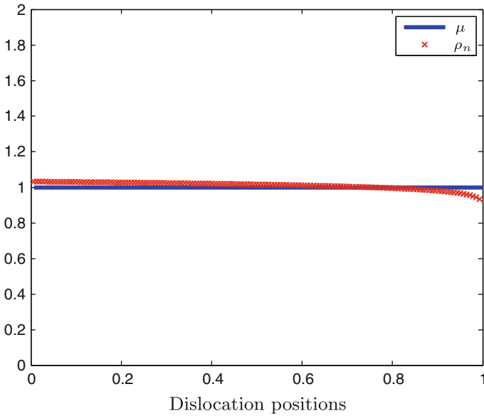
Fig. 7. Optimal densities relative to E_n^{(5)} and E^{(5)} , with n = 200 and \beta_n = 10^5
