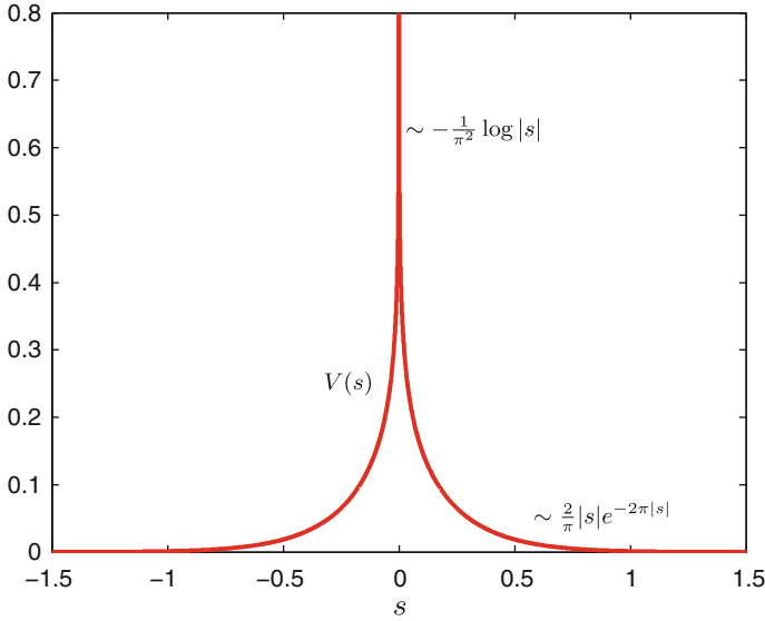
Fig. 2. The interaction energy V
