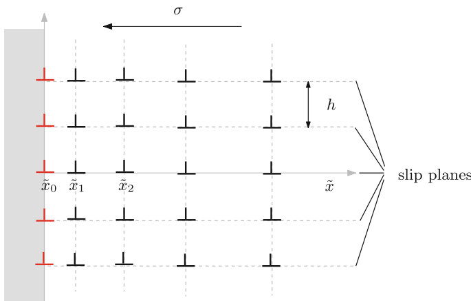
Fig. 1. The dislocation configuration considered in this paper. Infinite, vertical walls of equi-spaced dislocations are free to move in the horizontal direction. A wall of fixed dislocations is pinned at \tilde{x}_0 = 0 and acts as a repellent
