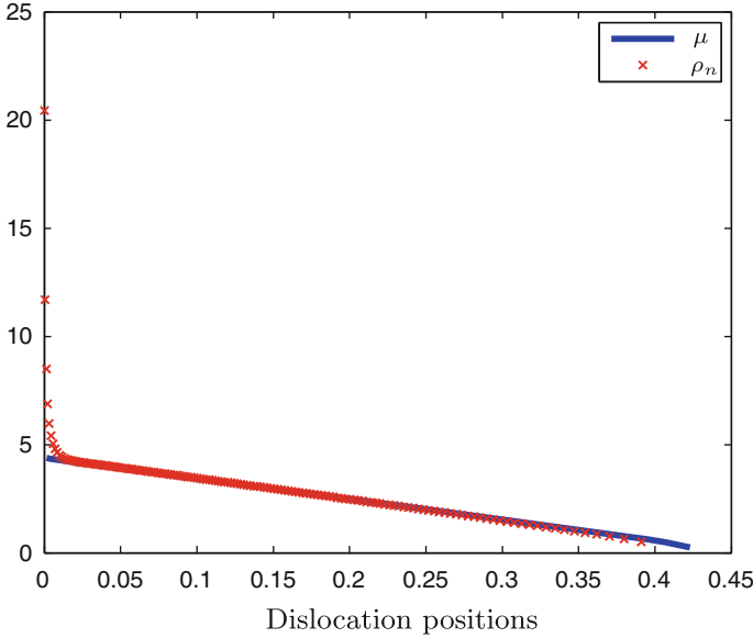
Fig. 5. Optimal densities relative to E_n^{(3)} and E^{(3)} , for n = 150 and \beta_n = 1/\sqrt{n} = 1/\sqrt{150}
