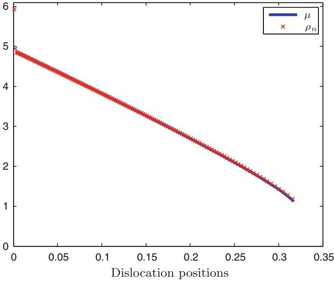
Fig. 6. Optimal densities relative to E_n^{(4)} and E^{(4)} , with n = 150 and \beta_n = 1
