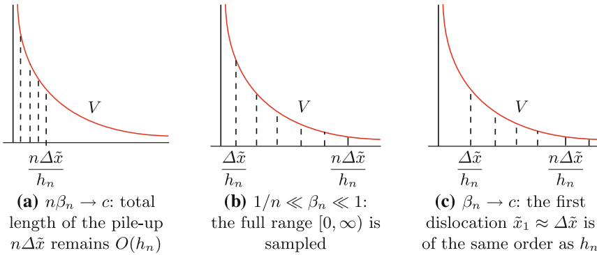
Fig. 8. Cases 2–4 of Theorem 1. Since \beta_n is a measure of the aspect ratio \Delta\tilde{x}/h_n , the scaling of \beta_n determines which values the ratio (\tilde{x}_i - \tilde{x}_j)/h_n takes in the argument of V in (1)
