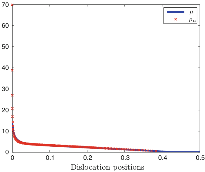
Fig. 4. Optimal densities relative to E_n^{(2)} and E^{(2)} , for n = 150 and \beta_n = 5/n
