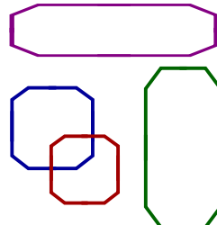
BeveledRects
