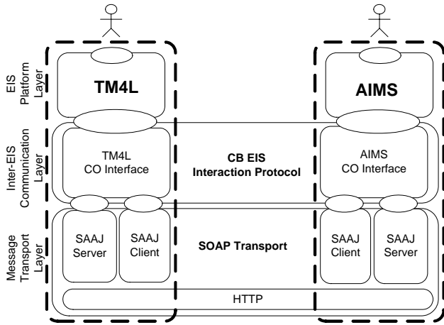
Figure 2. Minimalist integration framework for AIMS and TM4L
