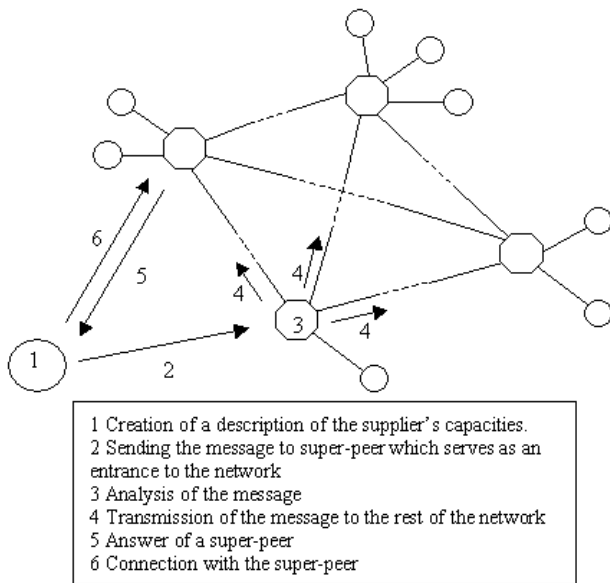
Figure 6. Connection of a New Edutella Supplier Peer Scenario
