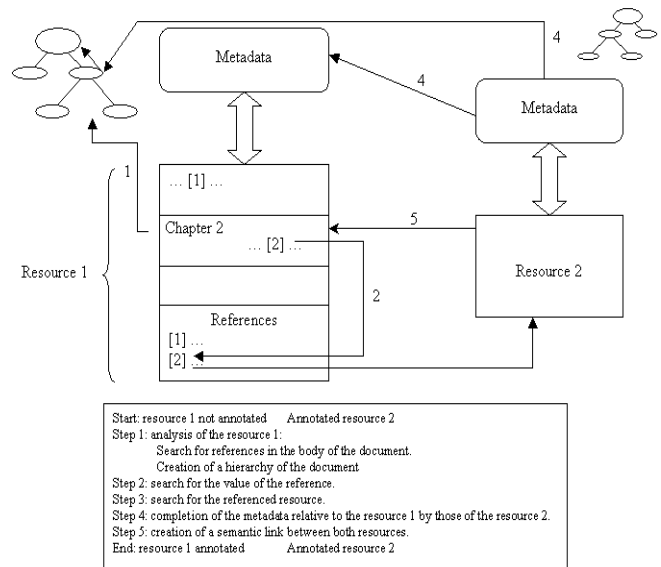
Figure 2. Annotation of learning objects: case n°1
