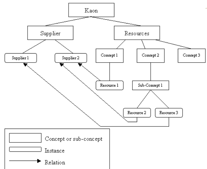
Figure 4. Example of an Ontology Model for Super-peers' Management
