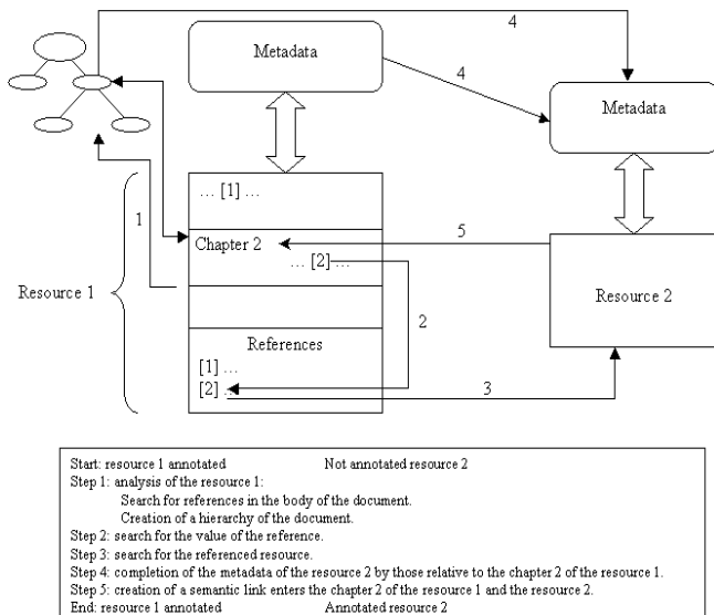
Figure 3. Annotation of learning objects: case n°2
