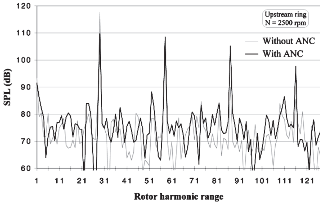
Figure 1. Measured spectra from test of new active control device for suppressing the blade passing tone due to interaction between rotor wakes and outlet guide vanes.
