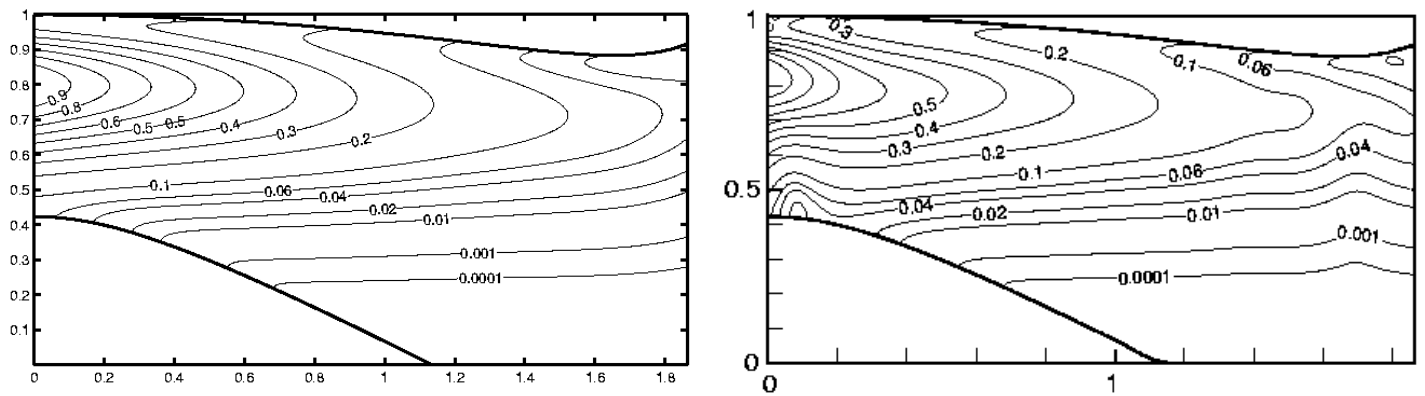
Figure 2. Iso-pressure contours from FEM (right) and multiple scales (left) solutions.
