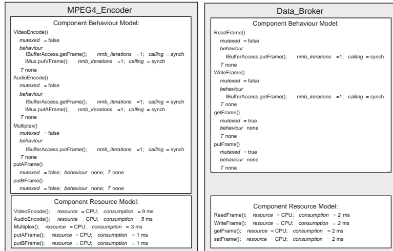
Fig. 16. Behaviour and resource models of the components from Fig. 15
