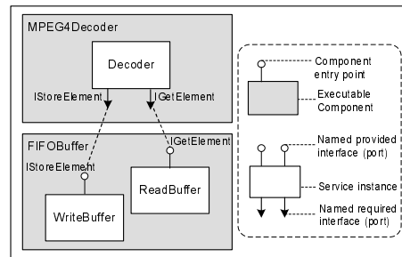
Fig. 10. Example of application structure
