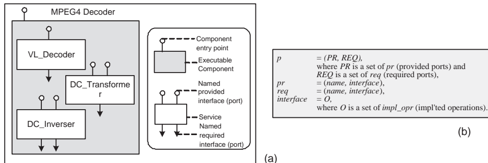
Fig. 3. (a) Example of executable component, (b) Specification of Robocop service
