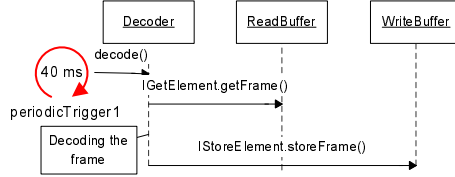
Fig. 11. Task triggered by in-application trigger
