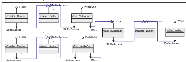
Fig. 17. Binding the encoder service instances
