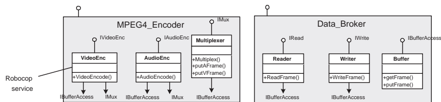
Fig. 15. Selected components with services, interfaces and operations
