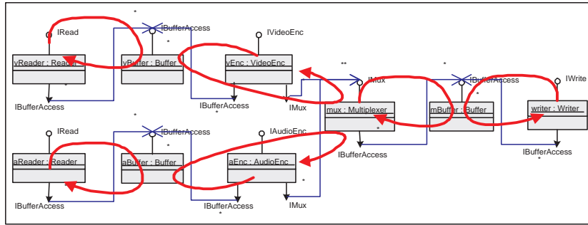
Fig. 20. Reconstructed tasks after models compilation
