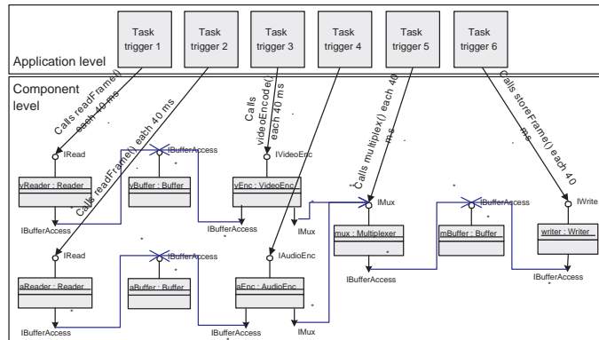
Fig. 18. Application level task triggers
