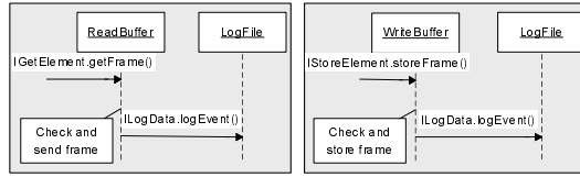
Fig. 12. The getFrame() and storeFrame() behaviour
