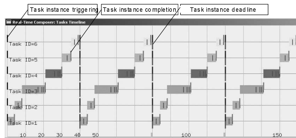
Fig. 21. Part of the task execution timeline for encoder application
