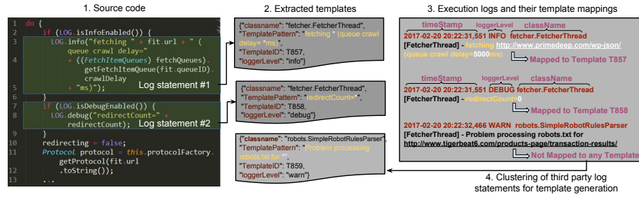
Fig. 2: Given the source code (1) templates are extracted (2), and log lines are mapped to them (3). Log lines from external libraries are clustered to create new templates (4).
