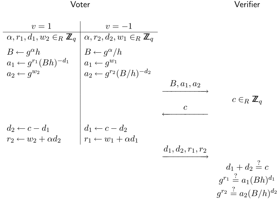
Figure 1: Encryption and Proof of Validity of Ballot B
