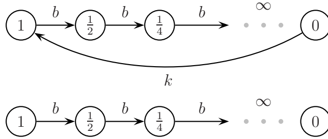
Fig. 4. Labelled transition systems for bouncing balls.
