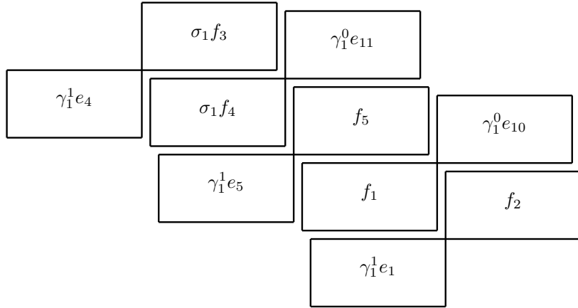
Fig. 5. A'' split up into five components.
