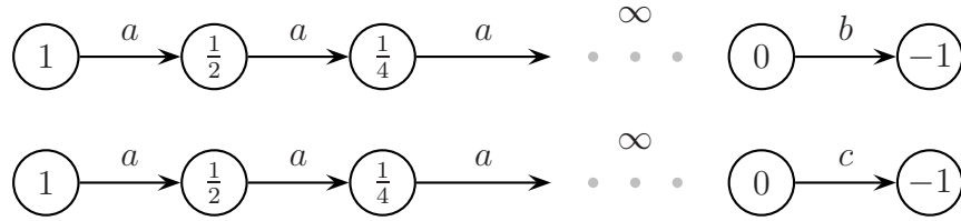
Fig. 2. Bisimilar labelled transition systems.
