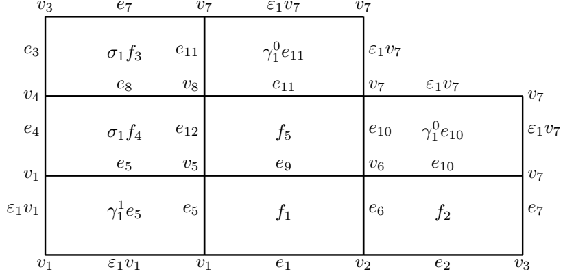
Fig. 2. A = \sigma_1 f_3 + \gamma_1^0 e_{11} + \sigma_1 f_4 + f_5 + \gamma_1^0 e_{10} + \gamma_1^1 e_5 + f_1 + f_2 : \partial^- A = e_1 + e_2 + e_7 , \partial^+ A = e_3 + e_4 + e_7 .
