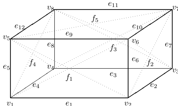
Fig. 1. The hollow 3-cube without bottom face.
