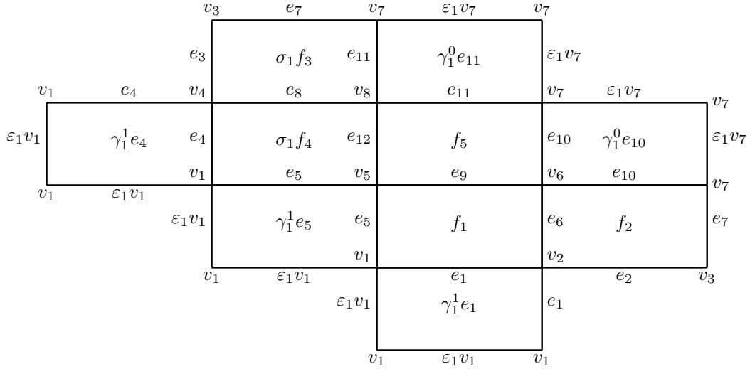
Fig. 4. A'' = A + \gamma_1^1 e_4 + \gamma_1^1 e_1 : \partial^- A'' = e_1 + e_2 + e_7 , \partial^+ A'' = e_3 + e_4 + e_7 , \zeta^- A'' = 5v_1 , \zeta^+ A'' = 5v_7 .
