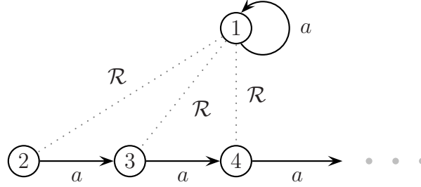
Fig. 5. A labelled transition system.
