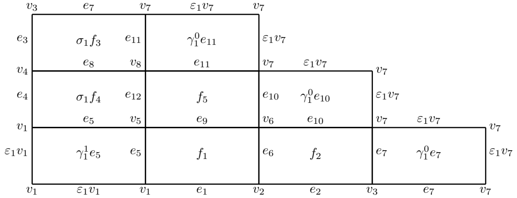
Fig. 2. A = \sigma_1 f_3 + \gamma_1^0 e_{11} + \sigma_1 f_4 + f_5 + \gamma_1^0 e_{10} + \gamma_1^1 e_5 + f_1 + f_2 : \partial^- A = e_1 + e_2 + e_7 , \partial^+ A = e_3 + e_4 + e_7 .
