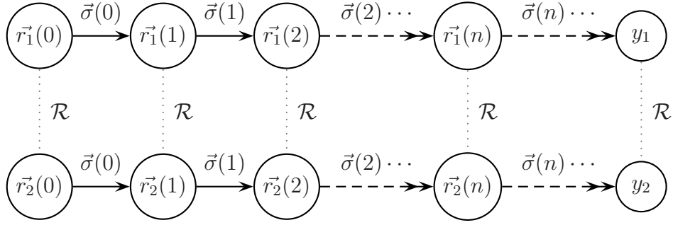
Fig. 3. Visualization of topological (bi-)simulation.
