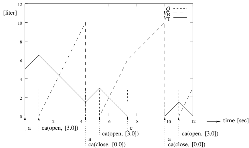
Fig. 2. Simulation results of model FillingLine .
