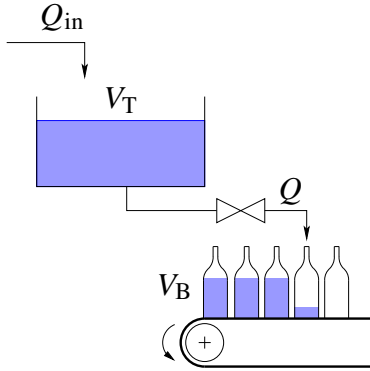
Fig. 1. Filling Line.
