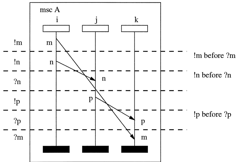
Fig. 3. Example MSC with separated events.
