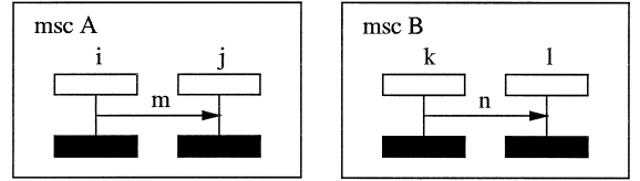
Fig. 7. Vertical composition with disjoint instances.
