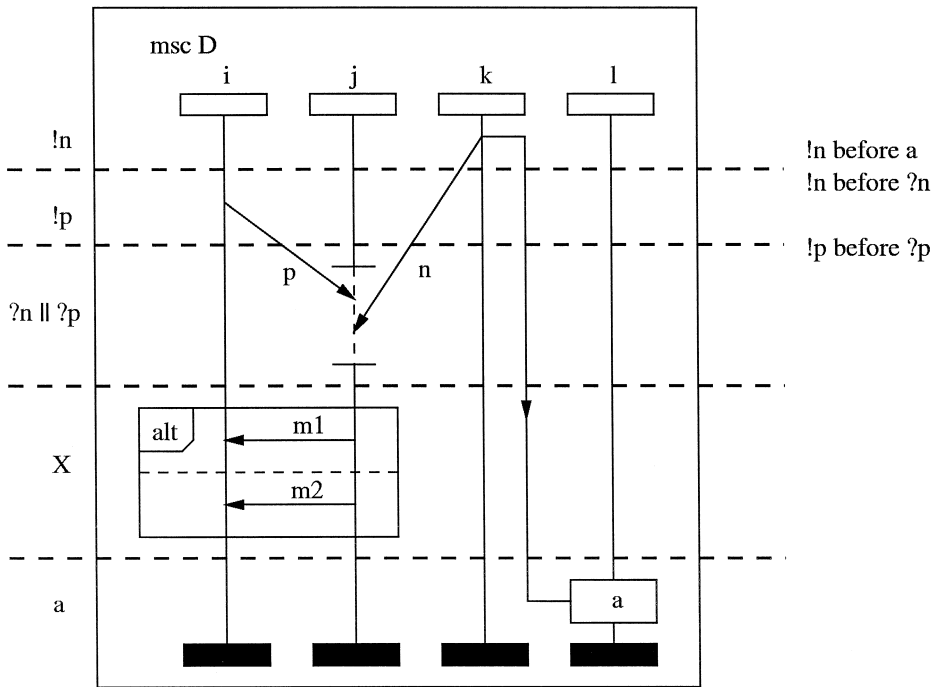
Fig. 6. Vertical decomposition of MSC D .
