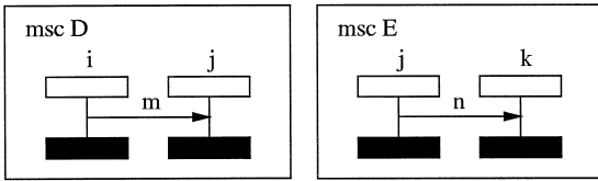
Fig. 8. Vertical composition with instances in common.
