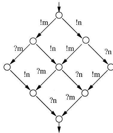
Fig. 9. Transition graph.
