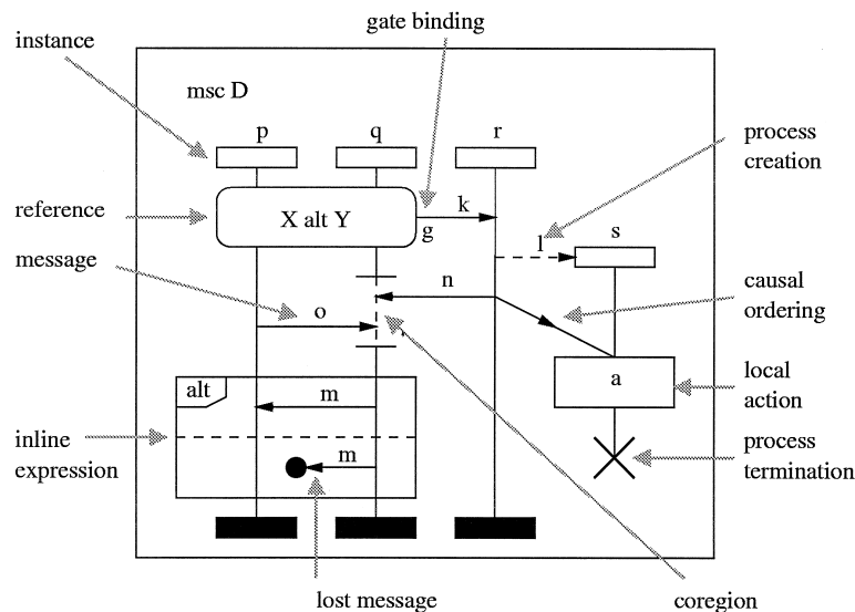
Fig. 1. Some MSC features.
