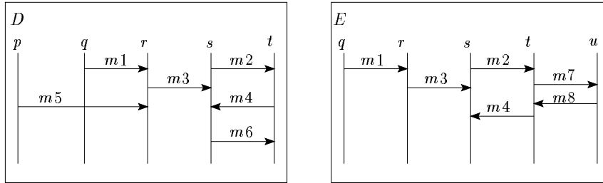
Fig. 2. Interworkings D (= A \circ_{iw} B) and E (= A \parallel_{iw} C)
