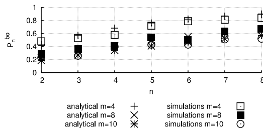
Fig. 7. Analytical and simulation results of the probability that node 4 is updated after the second Trickle interval, for different values of m ( I_{\min} = m \cdot w ).
