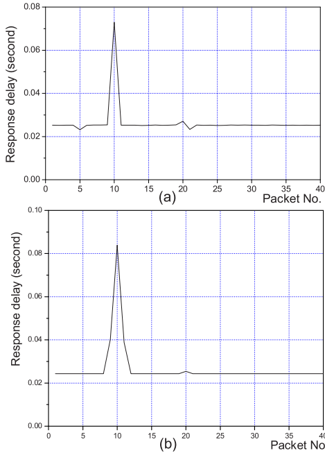
Fig. 3. The Response Delay of a Process Module
