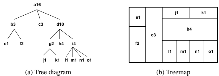
Fig. 1. Tree diagram
