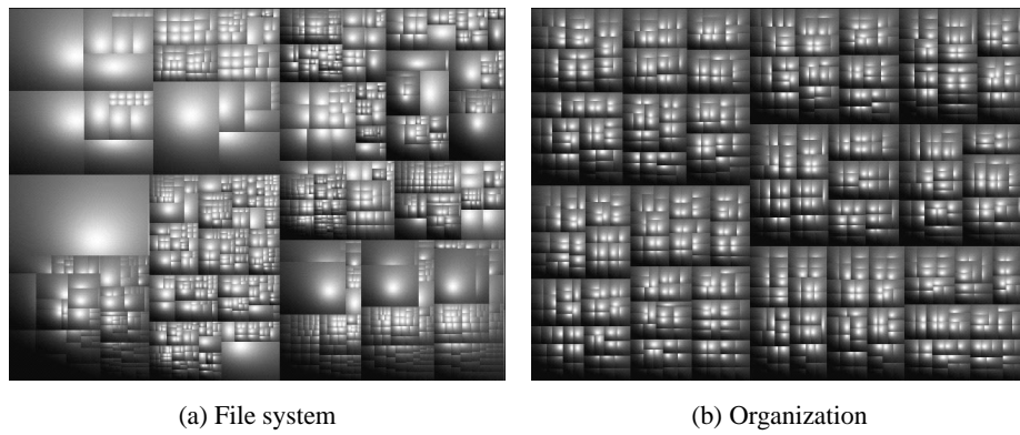
Fig. 5. Squarified treemaps
