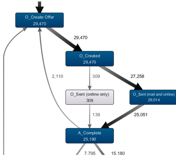
Fig. 5. Path diagram of sub-phase 1.2 Create Offer
