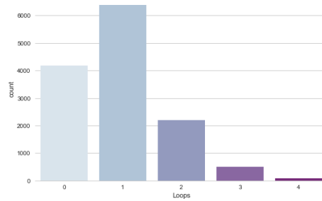
Fig. 16. Accepted cases per amount of loops
