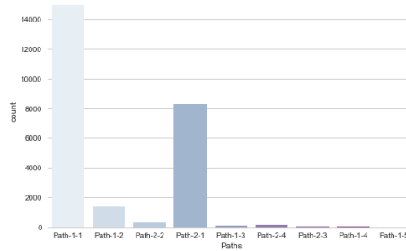
Fig. 10. Cases amount per path in Phase 1
