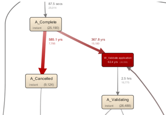
Fig. 3. Events waiting for an external input
