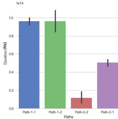
Fig. 11. Relation between duration and path for the most relevant paths in Phase 1
