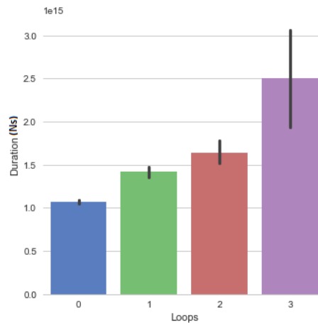
Fig. 19. Duration of Denied cases per amount of loops
