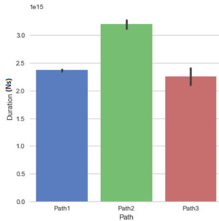
Fig. 14. Cases duration per path
