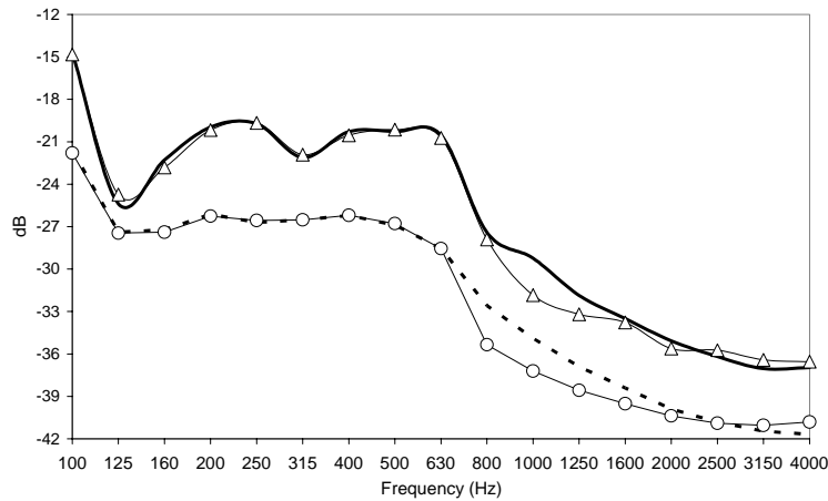
Figure 3.2: Power metric: Thick line, exact response, \eta=0.02 ; triangle, FEM and Scaled FEM, \eta=0.02 ; thick dashed line, exact response, \eta=0.10 ; circle, FEM and Scaled FEM, \eta=0.10
