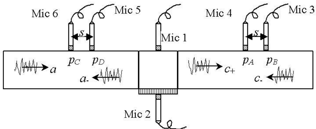
Figure 7.1: Impedance eduction measurement points
