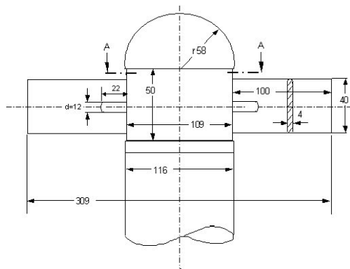
Figure 5.1: Technical drawing of the simplified propeller
