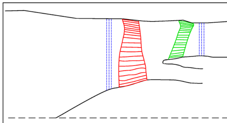
Figure 5.4: Sketch of triple-plane matching inlet and bypass geometry
