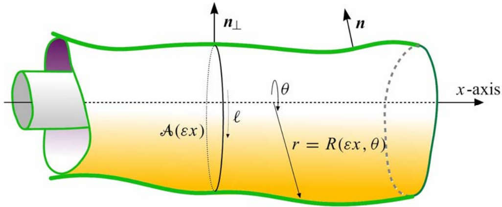
Figure 5.3: Sketch of slowly varying duct geometry
