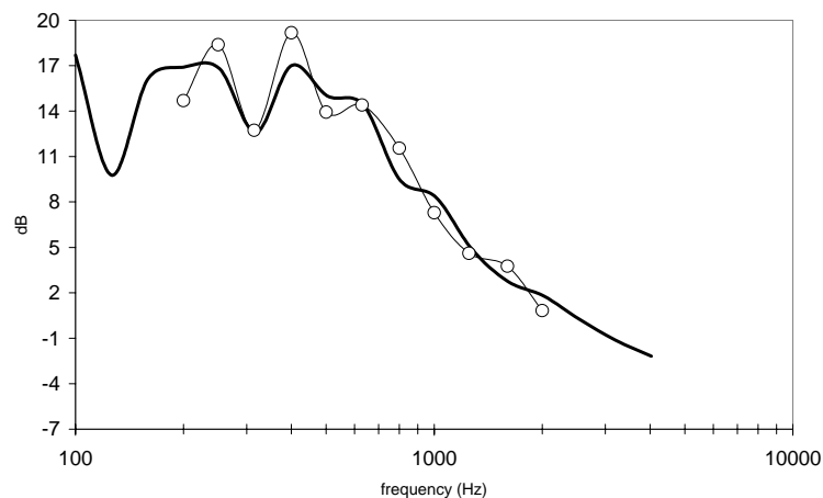
Figure 3.1: Structural metric: Thick line, exact response, \eta=0.02 ; circle, Scaled FEM, \eta=0.02
