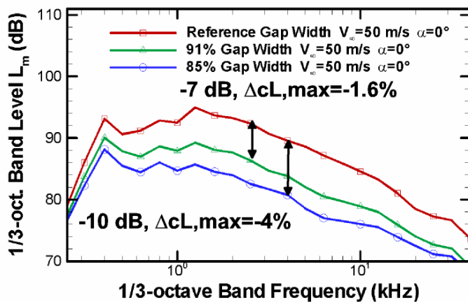
Figure 6.1: Effect of gap width on “as measured” slat noise spectra for 50m/s inflow speed and zero angle-of-attack
