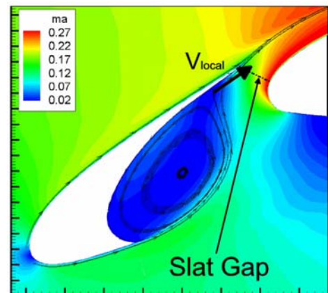
Figure 6.2: Mach number contours at a wing angle-of-attack of 4 deg and a slat deflection angle of 26 deg
