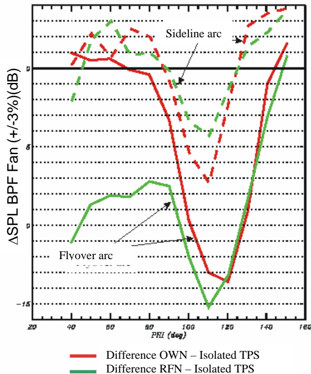
Figure 4.2: Shielding effect on the fan blade passage frequency (BPF) directivities for the OWN and RFN aircraft configurations. Difference SPL level versus Isolated TPS configuration. - RPM = 32500 - V_s = 60 m/s
