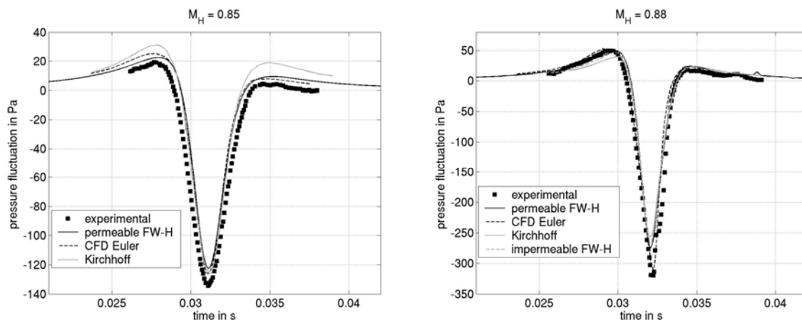
Figure 4.3: Noise for non lifting UH-1H blade in hover: M_H = 0.85 (left) and M_H = 0.88 (right)
