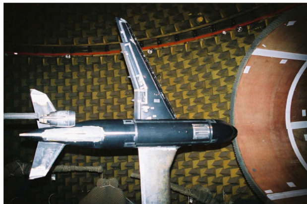
Figure 4.1: Fan noise test in ONERA CEPRA 19: ROSAS model and TPS nacelle, RFN layout
