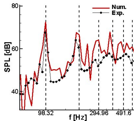
Figure 5.2: Experimental and numerical sound pressure level of the simplified propeller
