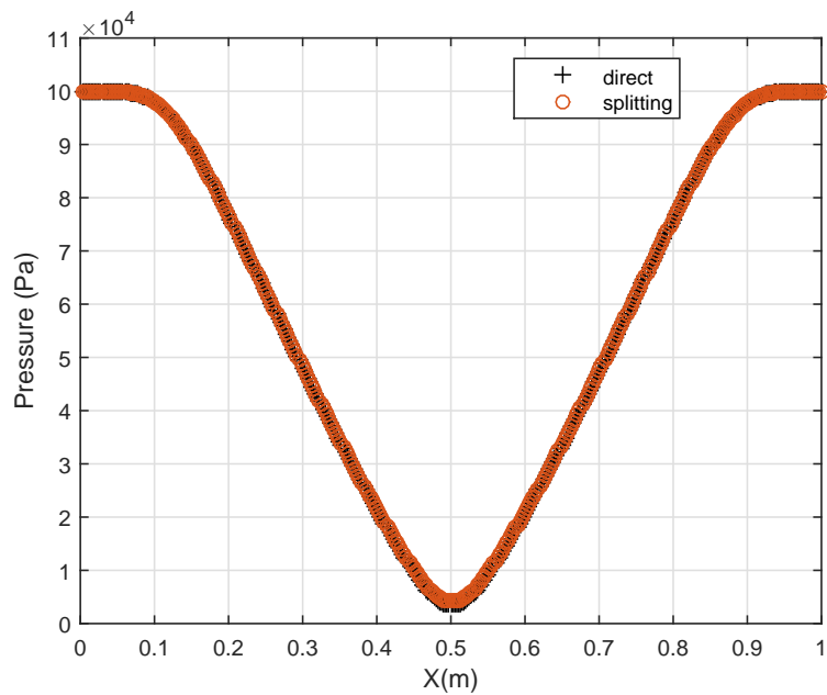
Figure 25: Two-phase cavitation problem problem - Pressure profile - Splitting approach “o” and direct approach “+” at t = 3.2 ms.
