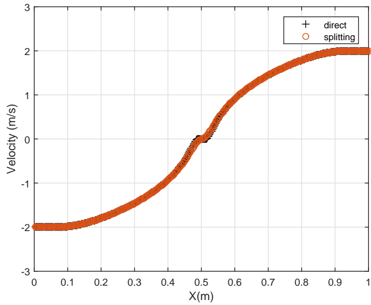
Figure 24: Two-phase cavitation problem problem - Velocity profile - Splitting approach “o” and direct approach “+” at t = 3.2 ms.
