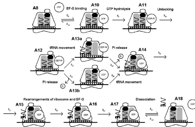
Fig. 3. Kinetic scheme of translocation taken from [7].
