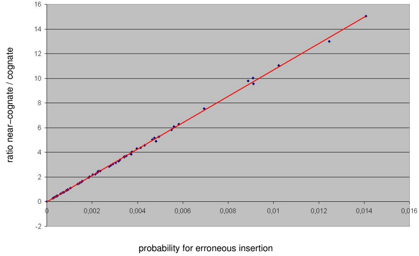
Fig. 4. Correlation of \frac{f_n}{f_c} ratio and error probabilities
