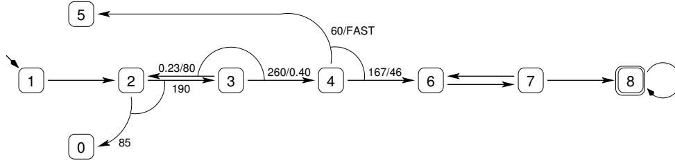
Fig. 1. Abstract automaton for error insertion
