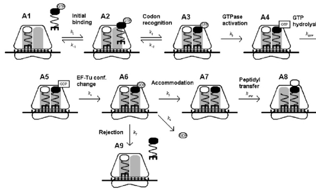
Fig. 2. Kinetic scheme of peptidyl transfer taken from [7].
