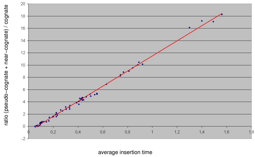
Fig. 5. Correlation of \frac{f_p+f_n}{f_c} ratio and average insertion times
