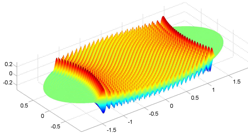
Figure 7: Eigenmode \psi_e^{41,25} for the ellipse with \alpha = 2 and \beta = 1 that has its eigenfrequency closest to \omega = 100 .
