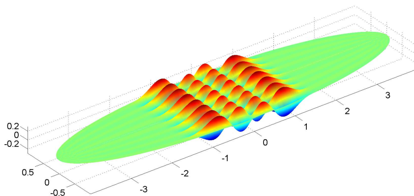
Figure 5: Eigenmode \psi_e^{3,8} for the ellipse with \alpha = 4 and \beta = 1 .
