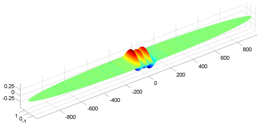
Figure 8: Eigenmode \psi_e^{6,1} for the ellipse with \alpha = 1000 and \beta = 1 .
