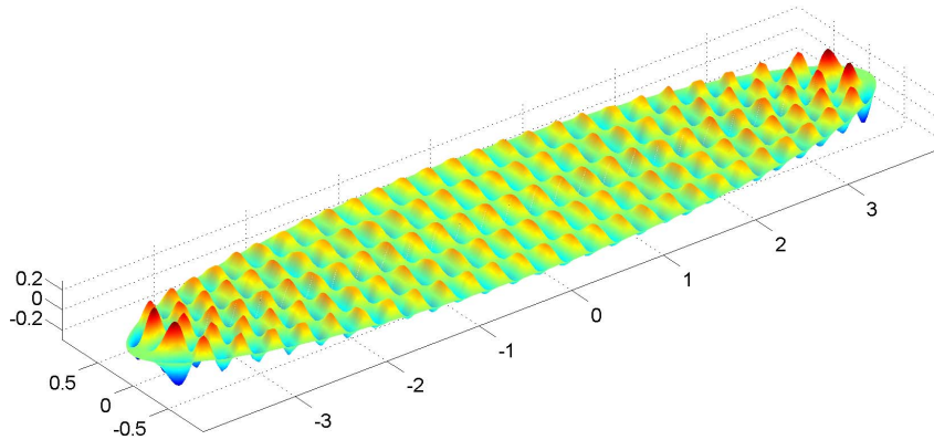
Figure 6: Eigenmode \psi_e^{52,3} for the ellipse with \alpha = 4 and \beta = 1 .
