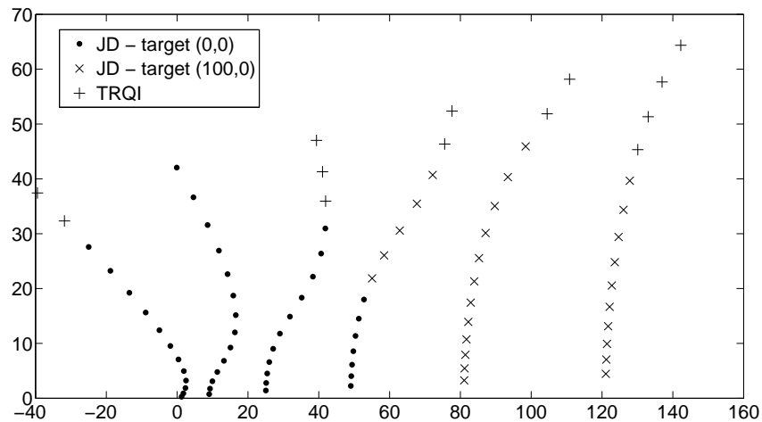
Figure 4: All eigenvalues of (1) with indices (i, j) for i \leq 13 and j \leq 5 , computed by the Jacobi–Davidson method using targets (0, 0) and (100, 0) , and extended by the TRQI.
