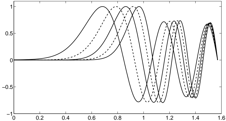
Figure 3: x -part of eigenvector of (14) corresponding to the eigenvalue with index (4, j) for j = 2, \dots, 6 .
