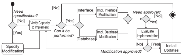
Fig. 6. Workflow of the software development process
