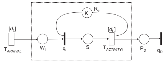
Fig. 2. Workflow System with a single activity
