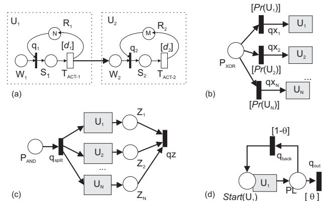
Fig. 3. Composition operations: a) SEQ; b) XOR; c) AND; d) LOOP
