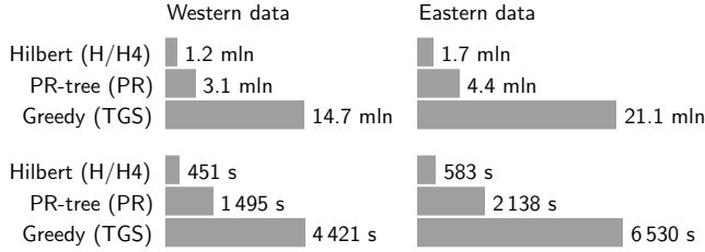
Figure 9: Bulk-loading performance on TIGER data: I/O (upper figure) and time (lower figure).
