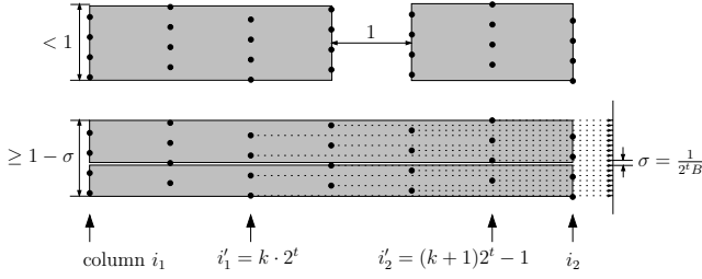
Figure 4: TGS partitioning the worst-case example. A vertical division creates two bounding boxes with a total area of less than i_2 - i_1 - 1 . A horizontal division creates two bounding boxes with a total area of more than (i_2 - i_1)(1 - 2\sigma) > i_2 - i_1 - 1 .
