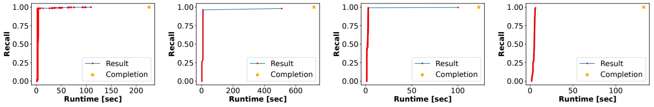
Fig. 9: Number of retrieved results over execution time, for progressive execution of queries on the Stocks dataset. (a) ES(1,3) query, \tau = 0.58 , \delta = 0.03 ; (b) MP(4) query, \tau = 0.8 , \delta = 0.05 ; (c) PC(1,3) query, \tau = 0.7 , \delta = 0.12 ; (d) TC(3) query, \tau = 0.25 , \delta = 1.3
