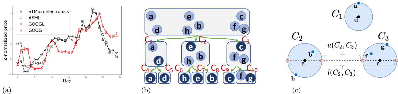
Fig. 2: (a) Two groups of closely related stocks: ASML and STMicroelectronics are exposed to similar risks, while GOOG and GOOGL participate in the same conglomeration; (b) Running example in 2 dimensions: the centroids of each cluster are depicted with darker background. All clusters are labeled for easy reference; (c) Illustration of pessimistic pairwise bounds of Lemma 1.
