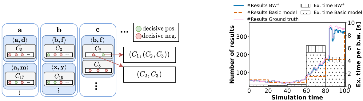
Fig. 4: (a) Visualization of the decisive combination index; (b) Number of results and execution time per basic window, with BW^+ and the standard basic window model. BW^+ is configured with epoch size 1. The results correspond to the Stocks dataset, with n = 1000 , w = 120000 , and b = 20 .
