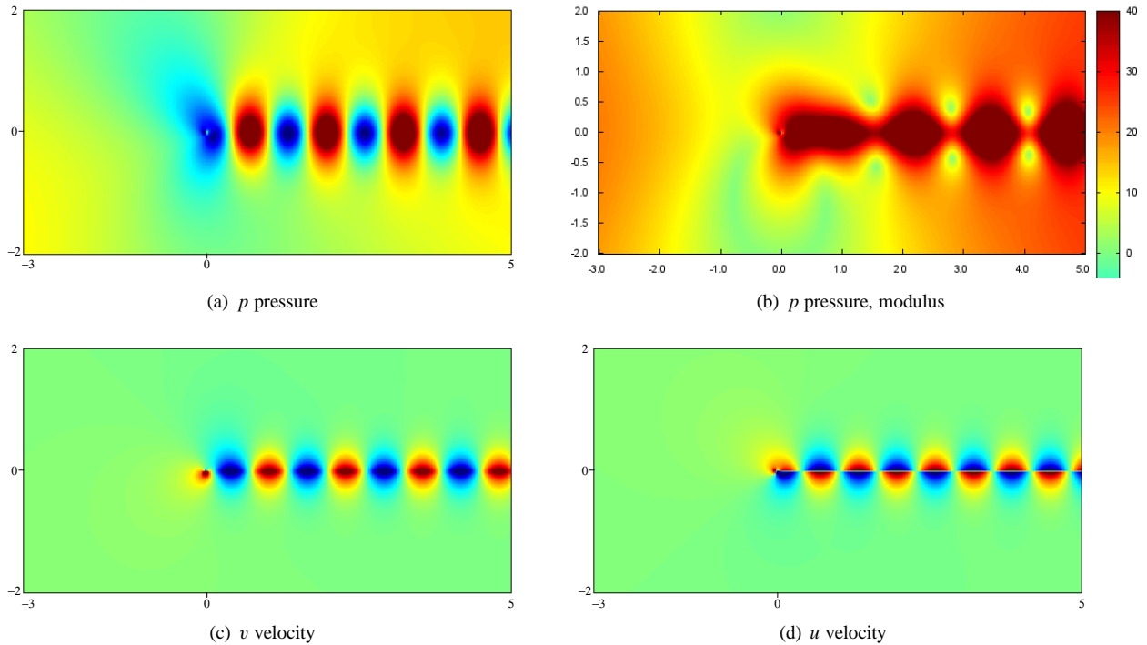
Figure 9. Pressure and velocity field of line source in incompressible linear mean shear flow for \omega = 10 , \sigma = 20 and U_0 = 2 , x \in [-3, 5] .
