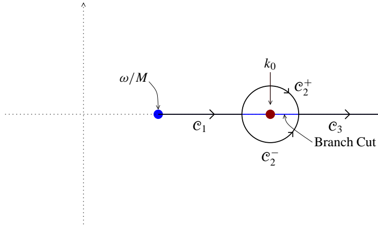
Figure 2. Schematic of the k -plane showing the Fourier inversion contour ( C_+'' from figure 1d) collapsed onto the critical layer branch cut. The case r_0 > 1 - h is shown, giving a pole at k = k_0 on the branch cut.
