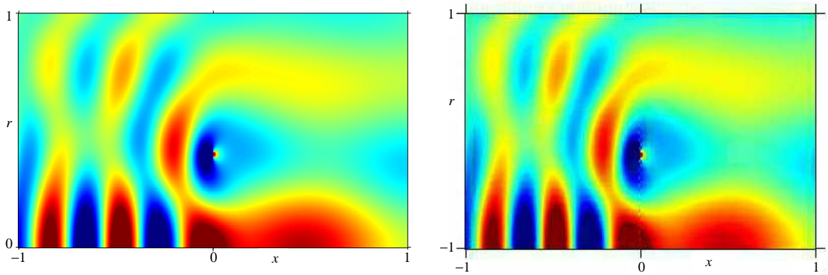
Figure 7. The Green's function with source in mean flow region for (left) uniform flow with Ingard-Myers condition; (right) constant-then-linear flow profile ( \omega = 10, m = 0, Z = 2 - i, h = 0.001, r_0 = 0.4 .)
