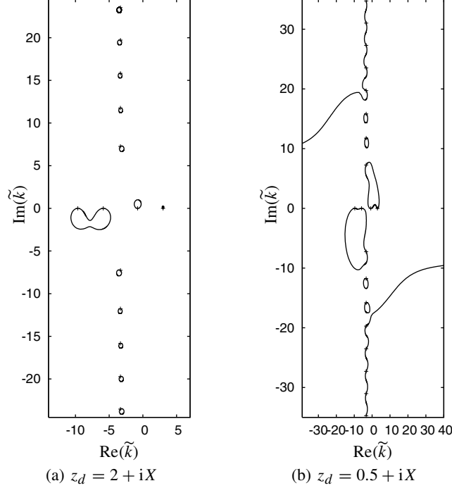
FIGURE 3. Trajectories of the axial wavenumber \tilde{k} for \tilde{\omega} = 5 , m = 1 , M = 0.5
