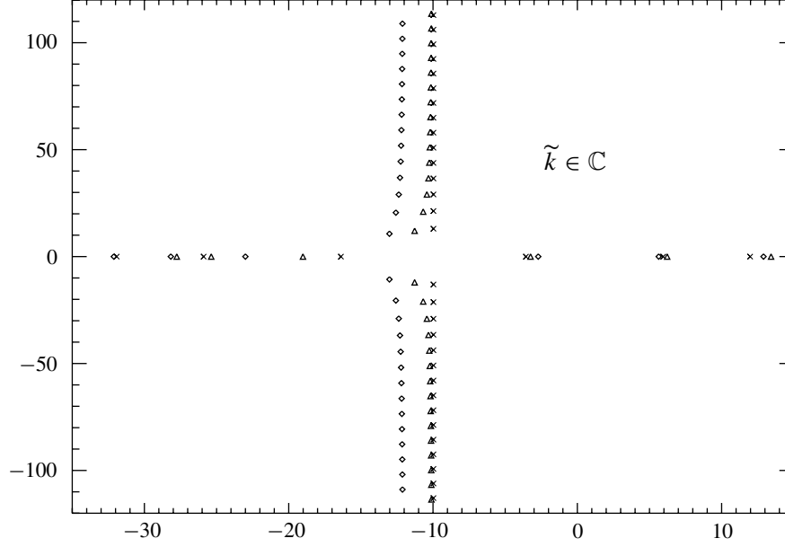
FIGURE 2. Effect of mean flow non-uniformity on the acoustic part of axial wavenumber spectrum, \tilde{\omega} = 25 , m = 15 , s = h/d = 0.5 . \times - uniform flow ( M = 0.35 ), \Delta - linear profile ( M_h = 0.5 , M_d = 0.2 ), \diamond - parabolic profile ( M_h = 0.5 , M_d = 0.2 ).
