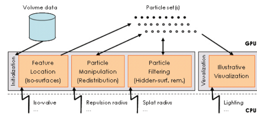
Figure 3: The VolFliesGPU framework.
